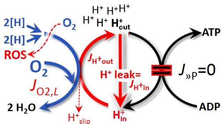
Fig. 5. LEAK state when phosphorylation is arrested, J_{\gg P}=0 , and oxygen flux, J_{O_2,L} , is controlled mainly by the proton leak, which equals J_{H^+_{in}} , at maximum \Delta p_{mt} (see also Fig. 2).
